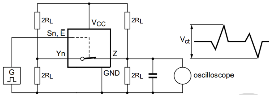
Figure 14. Test circuit for measuring crosstalk between control input and any switch
