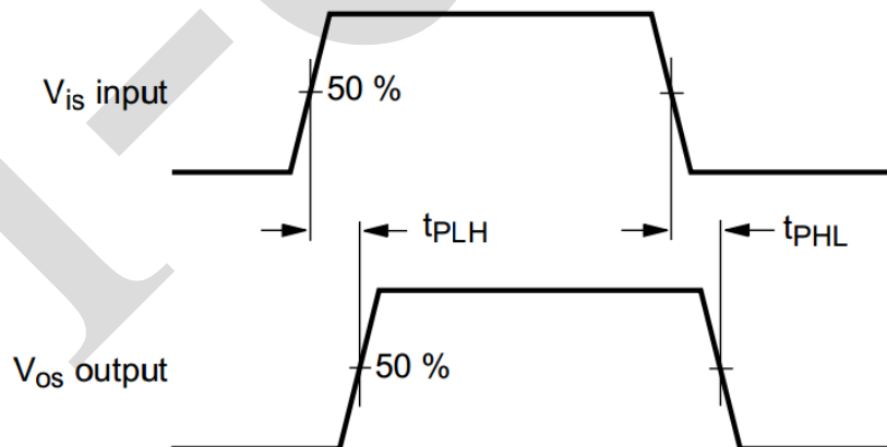
Figure 9. Input ( V_{is} ) to output ( V_{os} ) propagation delays
