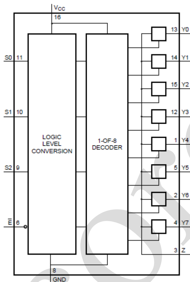
Figure 4. Functional diagram
