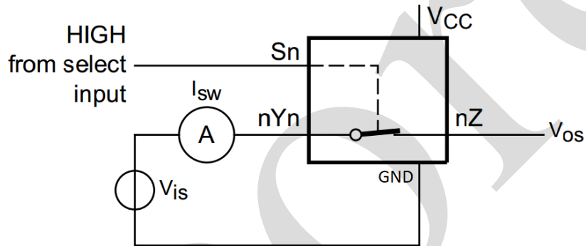
Figure 7. Test circuit for measuring OFF-state current
